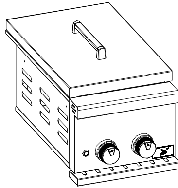
PERSPECTIVE VIEW
